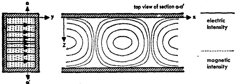
Fig. 2—Field configuration for TE_{0,1} wave.
