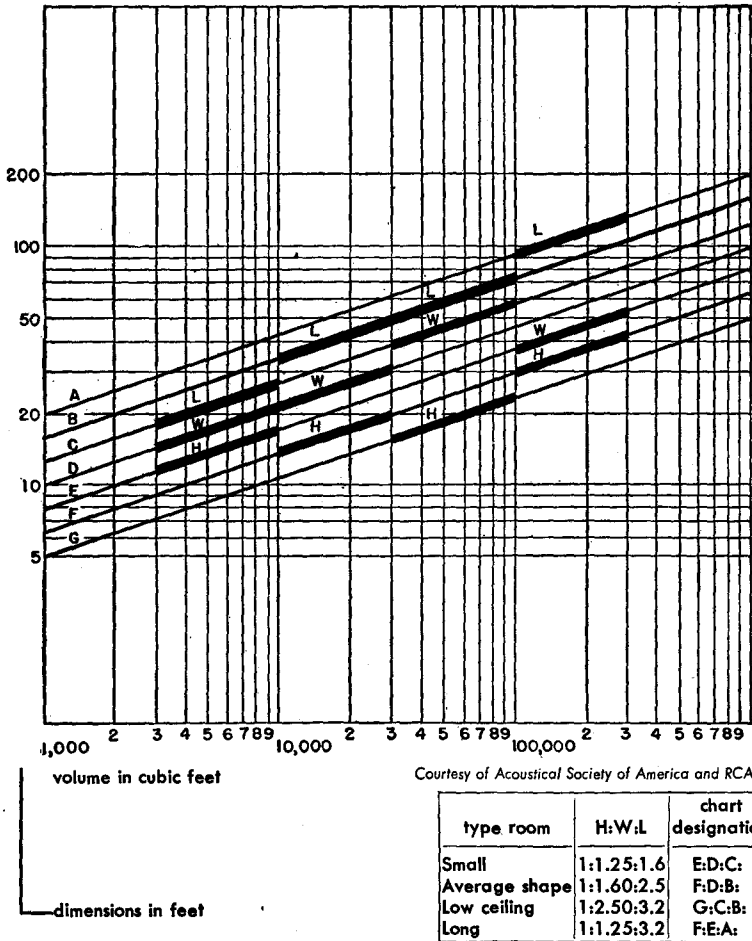
Fig. 1—Preferred room dimensions based on 2^1 ratio. Permissible deviation \pm 5 percent.
