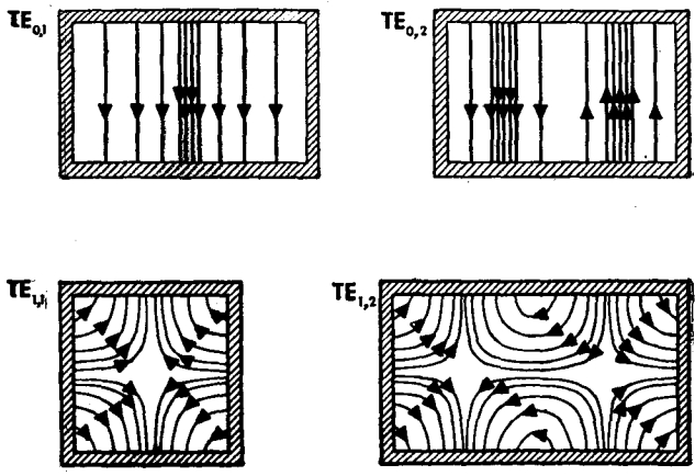
Fig. 4—Characteristic E lines for TE waves.
